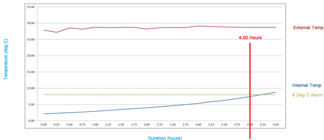
Polartherm Clamshell Bag Temperature Performance
